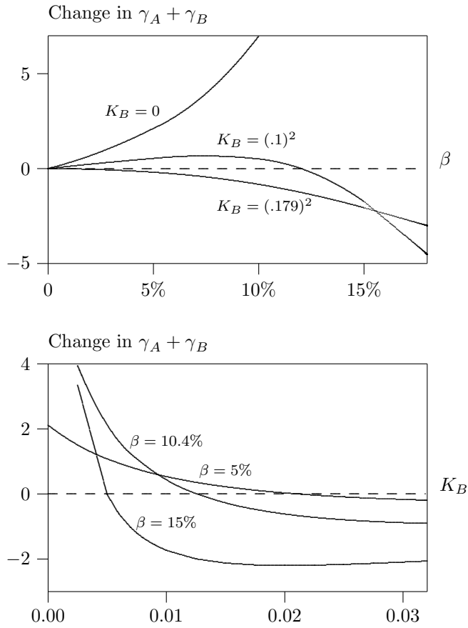
Figure 1: BSkyB's divestiture of its partial holding on ITV (by means of a sale to small shareholders). Effect on \gamma_A + \gamma_B as a function of \beta for given values of K_B ; and as a function of K_B for given values of \beta . Recall that \gamma_A + \gamma_B is a sufficient statistic of consumer surplus: higher \gamma_A + \gamma_B implies lower consumer surplus.
