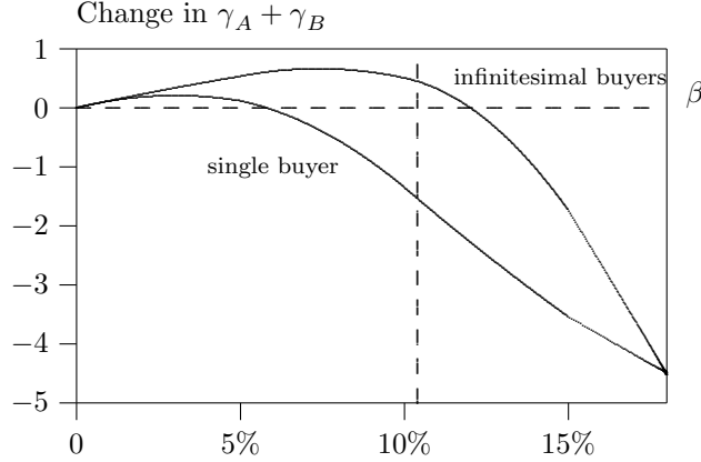
Figure 2: BSkyB’s divestiture of its partial holding on ITV. Effect on \gamma_A + \gamma_B as a function of \beta for K_B = .01 and assuming different types of buyers: one single large buyer and an infinite number of infinitesimal buyers.
